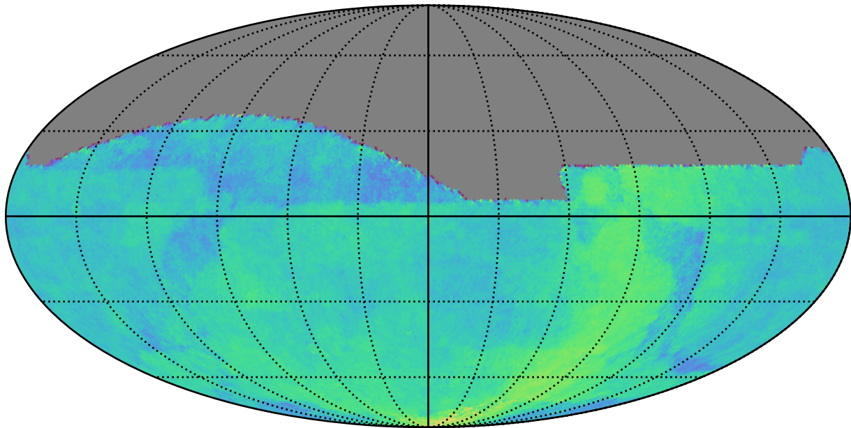
ddf_acor_sf15_lsf30_lsr50_v3.4_10yrs : Parallax Coverage @ 24.0
