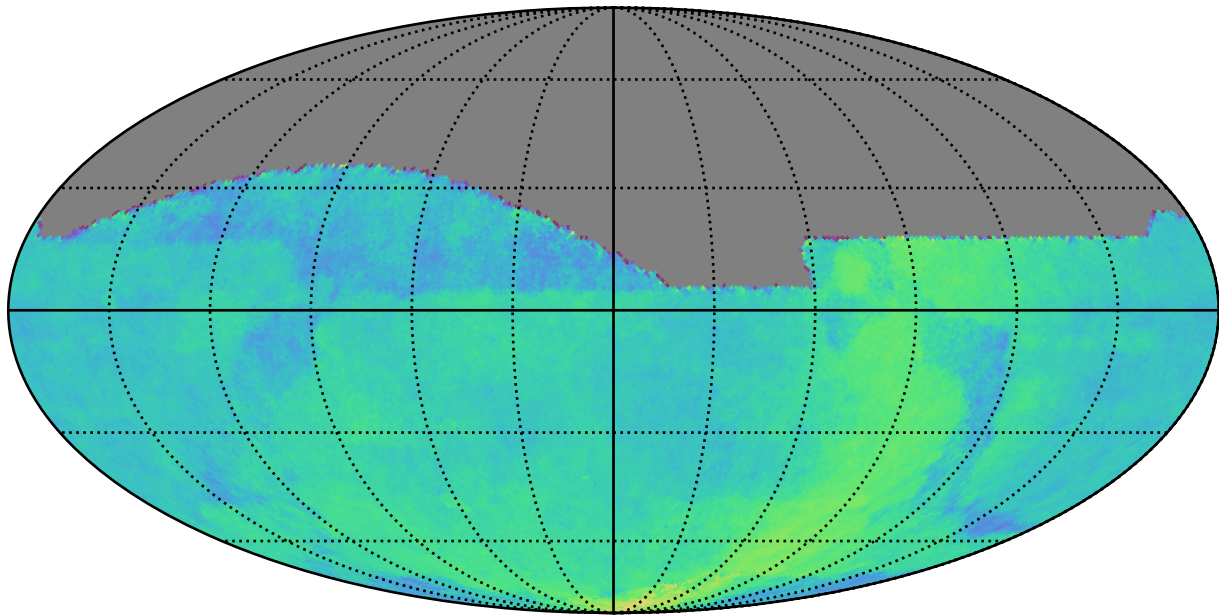
ddf_acor_sf15_lsf30_lsr50_v3.4_10yrs : Parallax Coverage @ 22.4
