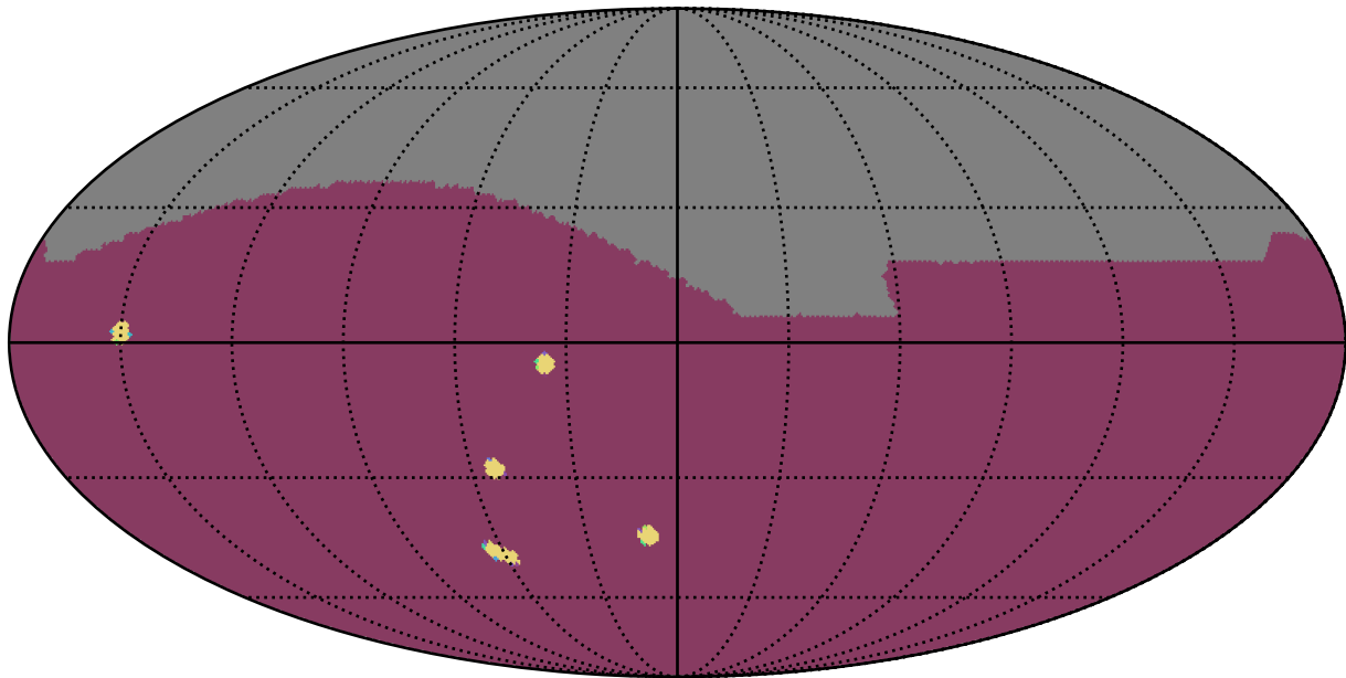
ddf_acor_sf15_lsf30_lsr50_v3.4_10yrs : NumberOfQuickRevisits
