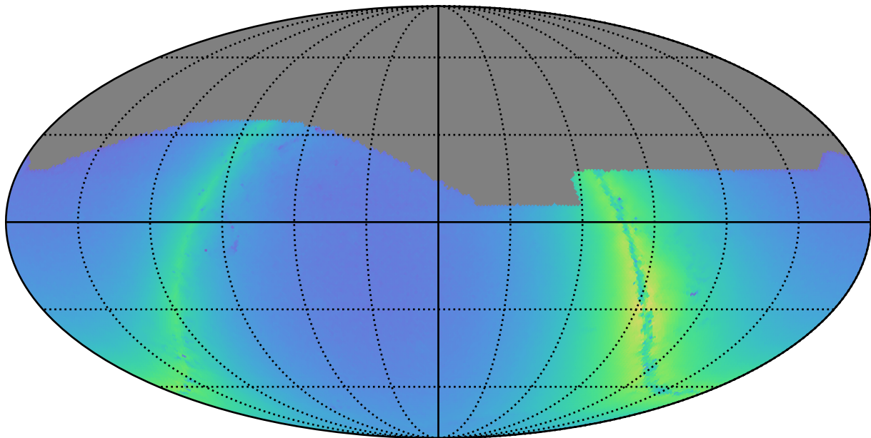
ddf_acor_sf15_lsf30_lsr50_v3.4_10yrs r: Nstars_no_crowding
