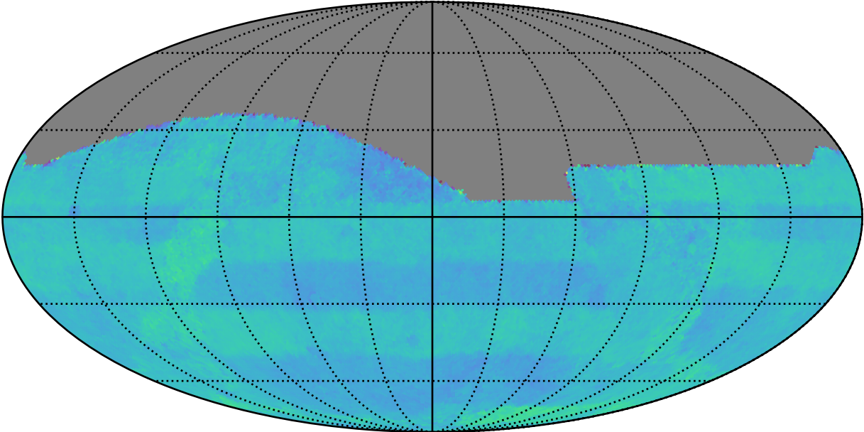
ddf_acor_sf15_lsf30_lsr50_v3.4_10yrs : Normalized Proper Motion Uncert @ 24.0
