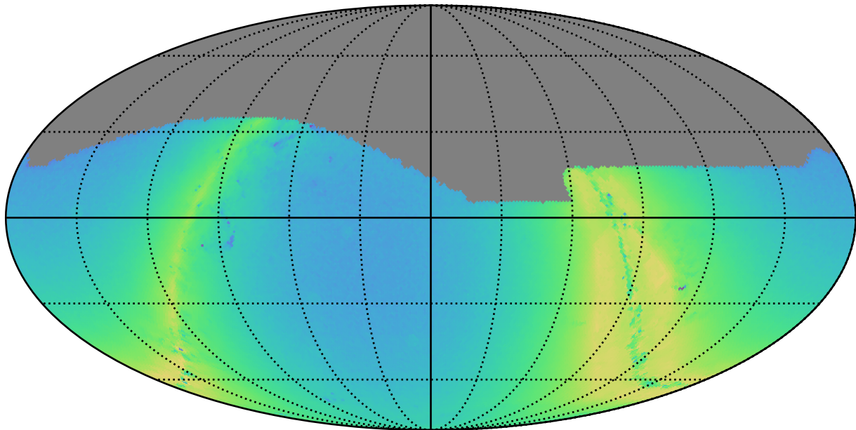
ddf_acor_sf15_lsf30_lsr50_v3.4_10yrs g: N stars to Precision 0.20
