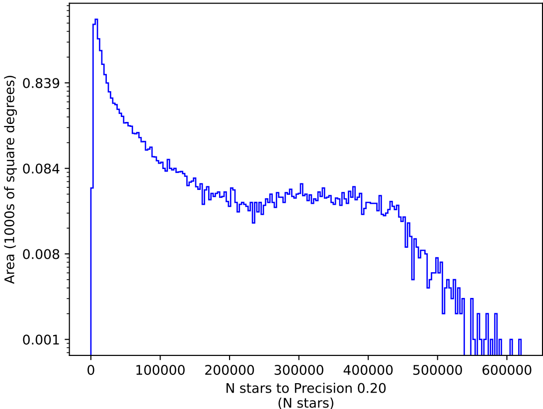
ddf_acor_sf15_ls30_lsr50_v3.4_10yrs g: N stars to Precision 0.20
