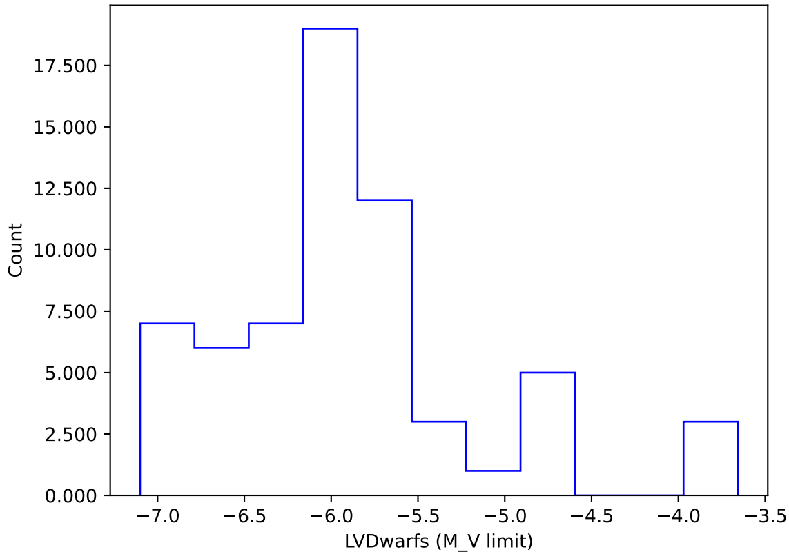
ddf_acor_sf15_lsf30_lsr50_v3.4_10yrs gi: LVDwarfs
