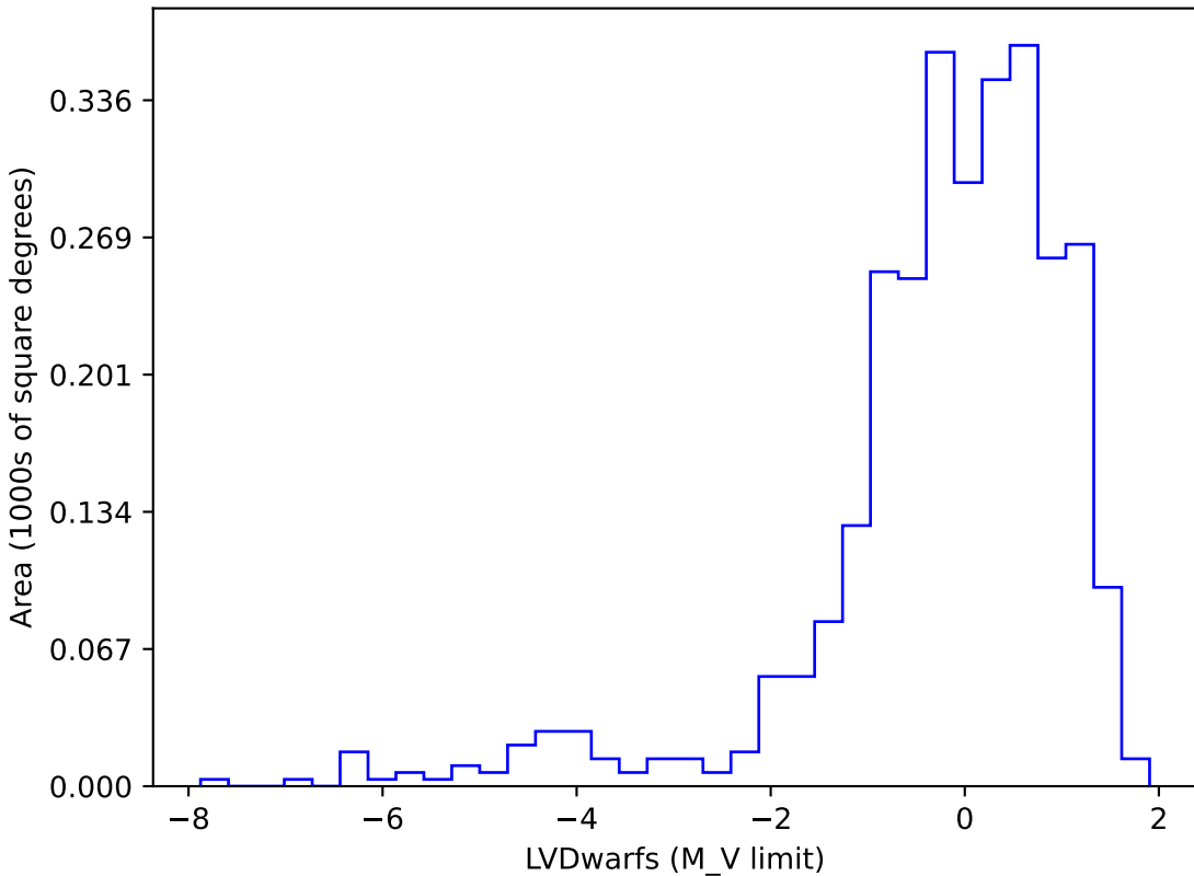
ddf_acor_sf15_lsf30_lsr50_v3.4_10yrs gi SCP: LVDwarfs
