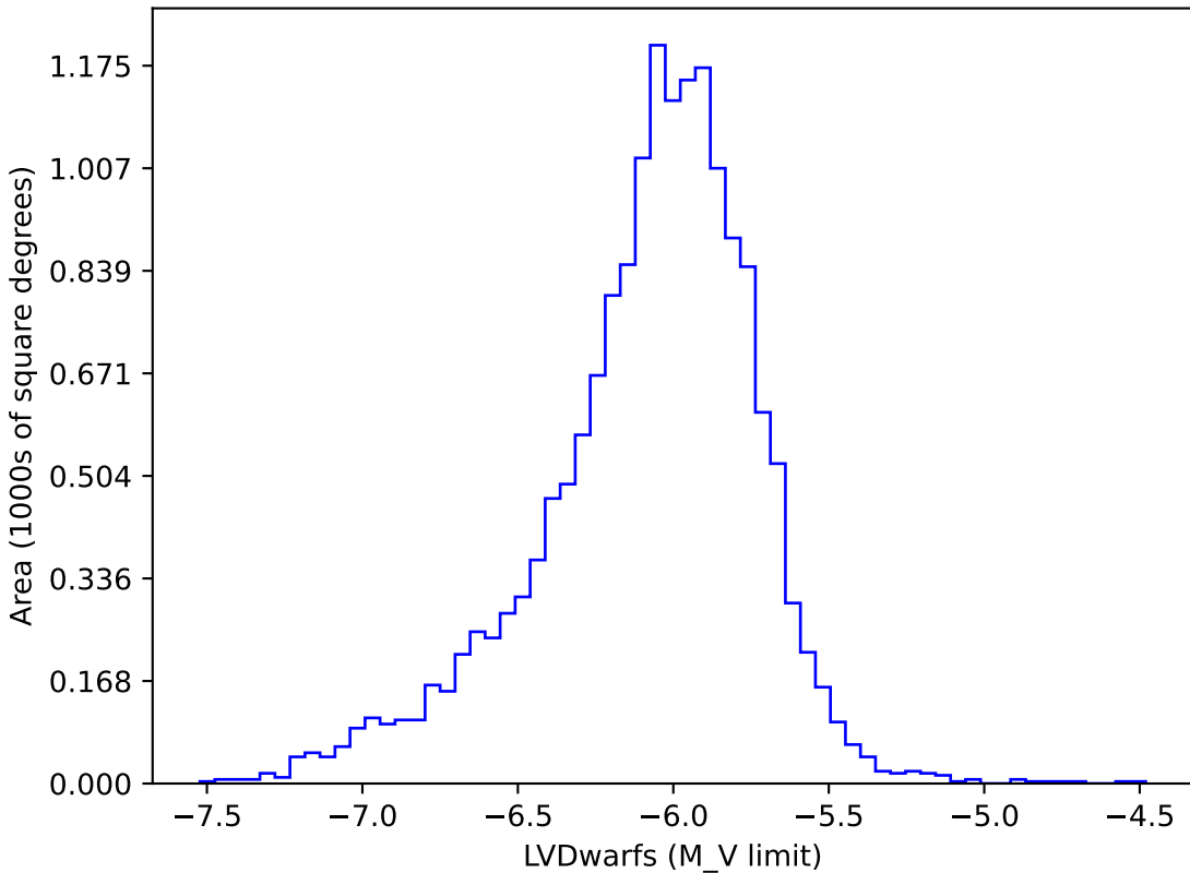
ddf_acor_sf15_lsf30_lsr50_v3.4_10yrs gi: LVDwarfs
