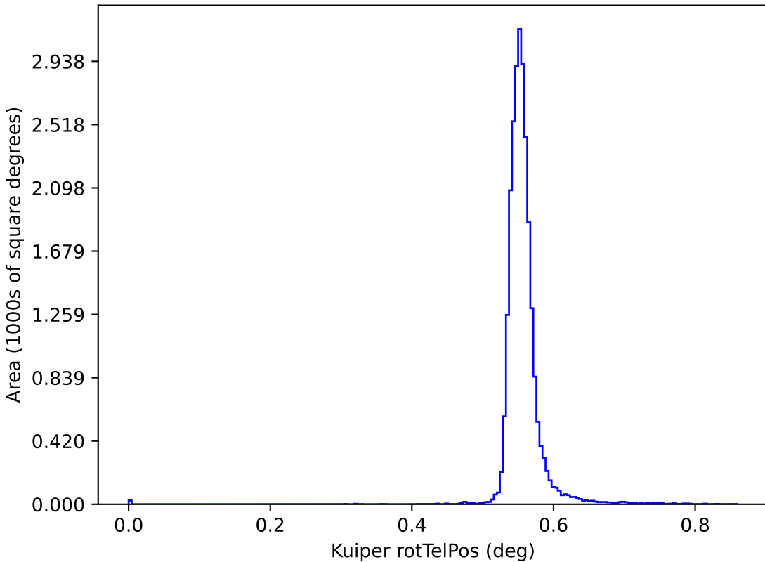
ddf_acor_sf15_lsf30_lsr50_v3.4_10yrs y: Kuiper rotTelPos
