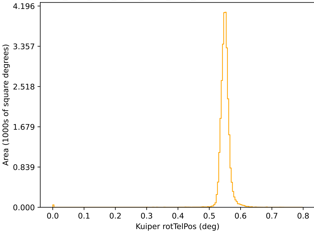
ddf_acor_sf15_lsf30_lsr50_v3.4_10yrs r: Kuiper rotTelPos
