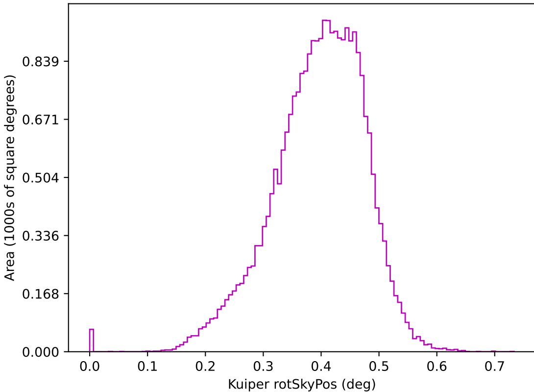
ddf_acor_sf15_lsf30_lsr50_v3.4_10yrs z: Kuiper rotSkyPos
