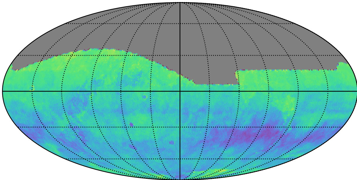
ddf_acor_sf15_lsf30_lsr50_v3.4_10yrs r: Kuiper rotSkyPos
