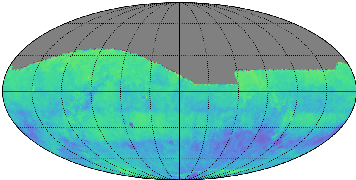
ddf_acor_sf15_lsf30_lsr50_v3.4_10yrs i: Kuiper rotSkyPos
