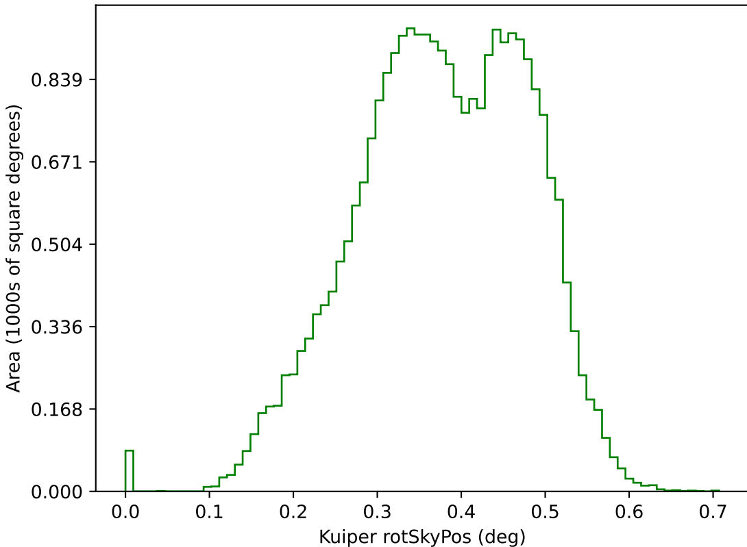
ddf_acor_sf15_lsf30_lsr50_v3.4_10yrs g: Kuiper rotSkyPos
