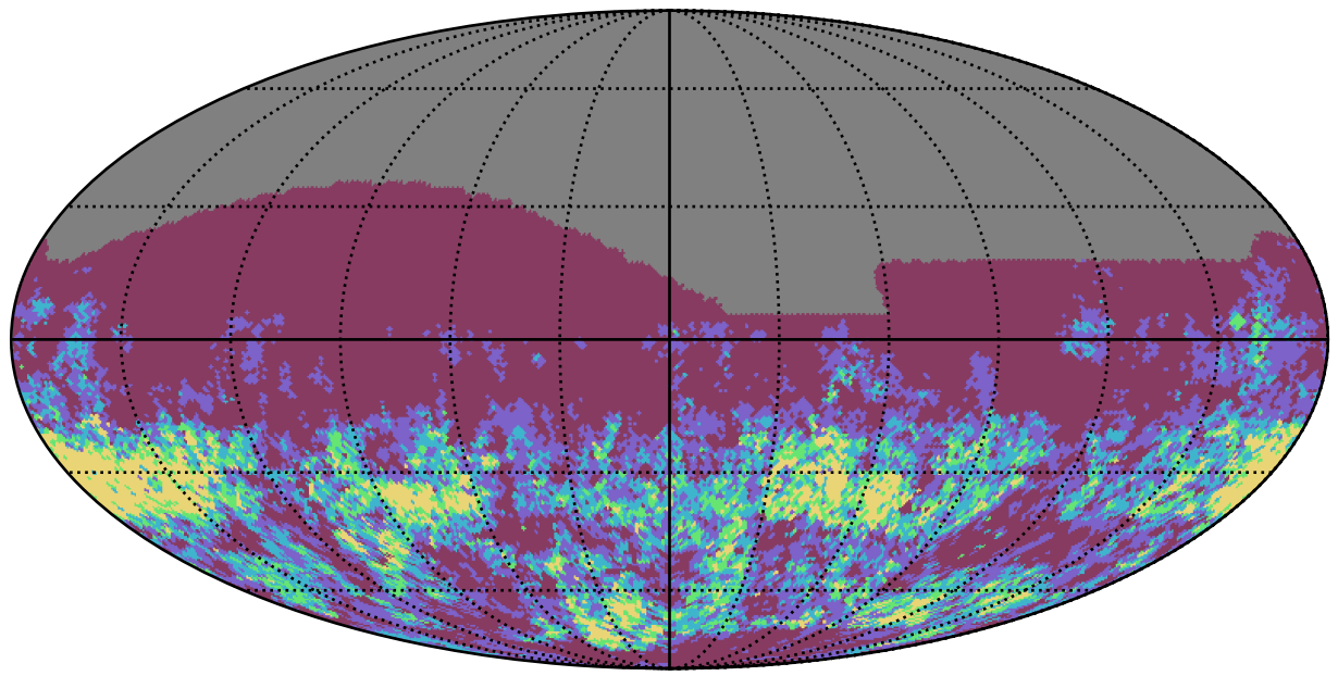
ddf_acor_sf15_lsf30_lsr50_v3.4_10yrs r band: Gaps_7hr
