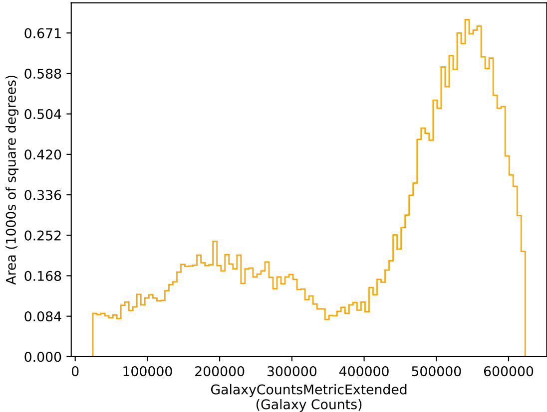
ddf_acor_sf15_lsf30_lsr50_v3.4_10yrs r: GalaxyCountsMetricExtended
