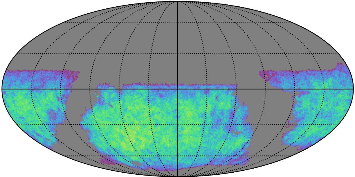
ddf_acor_sf15_lsf30_lsr50_v3.4_10yrs i band non-DD year 1: ExgalM5WithCuts
