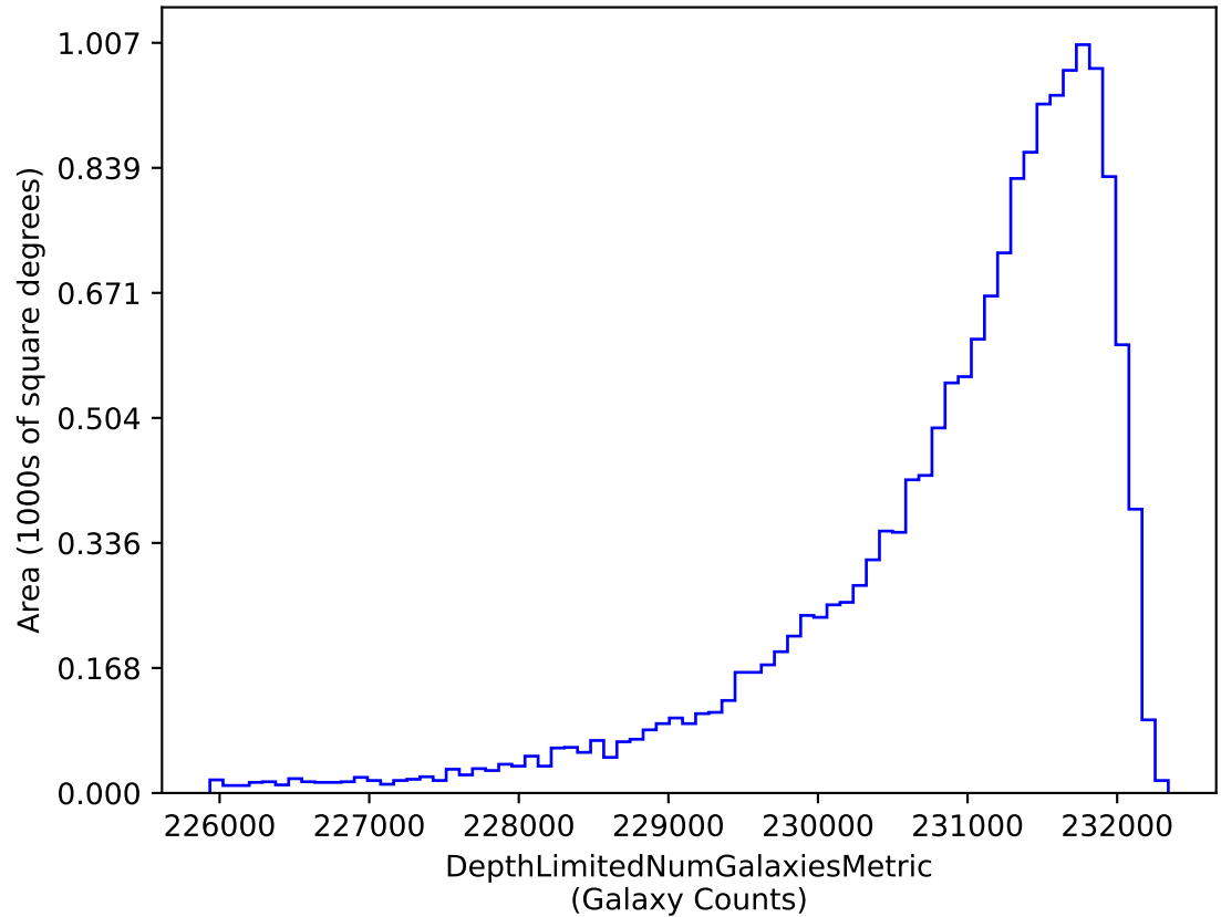
ddf_acor_sf15_lsf30_lsr50_v3.4_10yrs i band galaxies non-DD: DepthLimitedNumGalaxiesMetric
