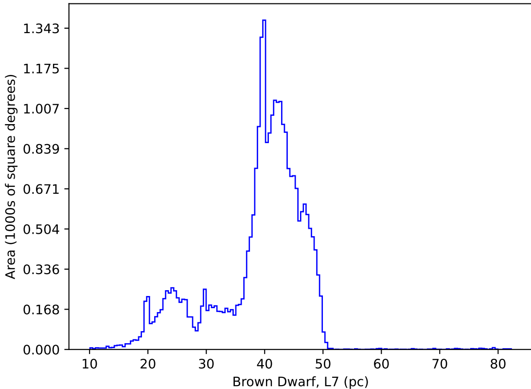
ddf_acor_sf15_lsf30_lsr50_v3.4_10yrs : Brown Dwarf, L7
