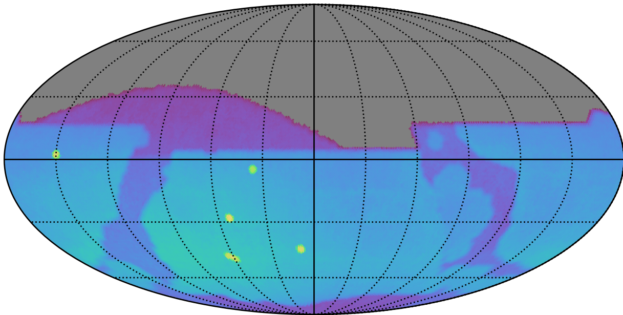
ddf_acor_sf15_lsf30_lsr50_v3.4_10yrs : Brown Dwarf, L4
