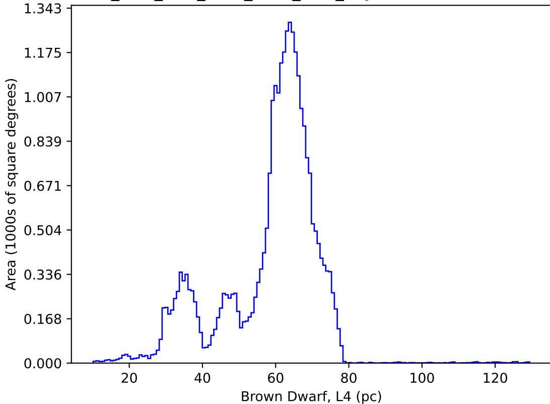
ddf_acor_sf15_lsf30_lsr50_v3.4_10yrs : Brown Dwarf, L4
