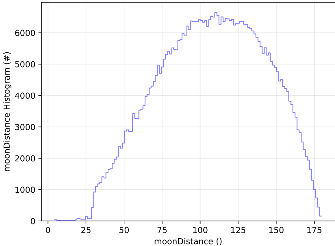
ddf_acor_sf15_lsf30_lsr50_v3.4_10yrs WFD r band: moonDistance Histogram
