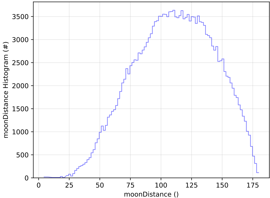
ddf_acor_sf15_lsf30_lsr50_v3.4_10yrs WFD g band: moonDistance Histogram
