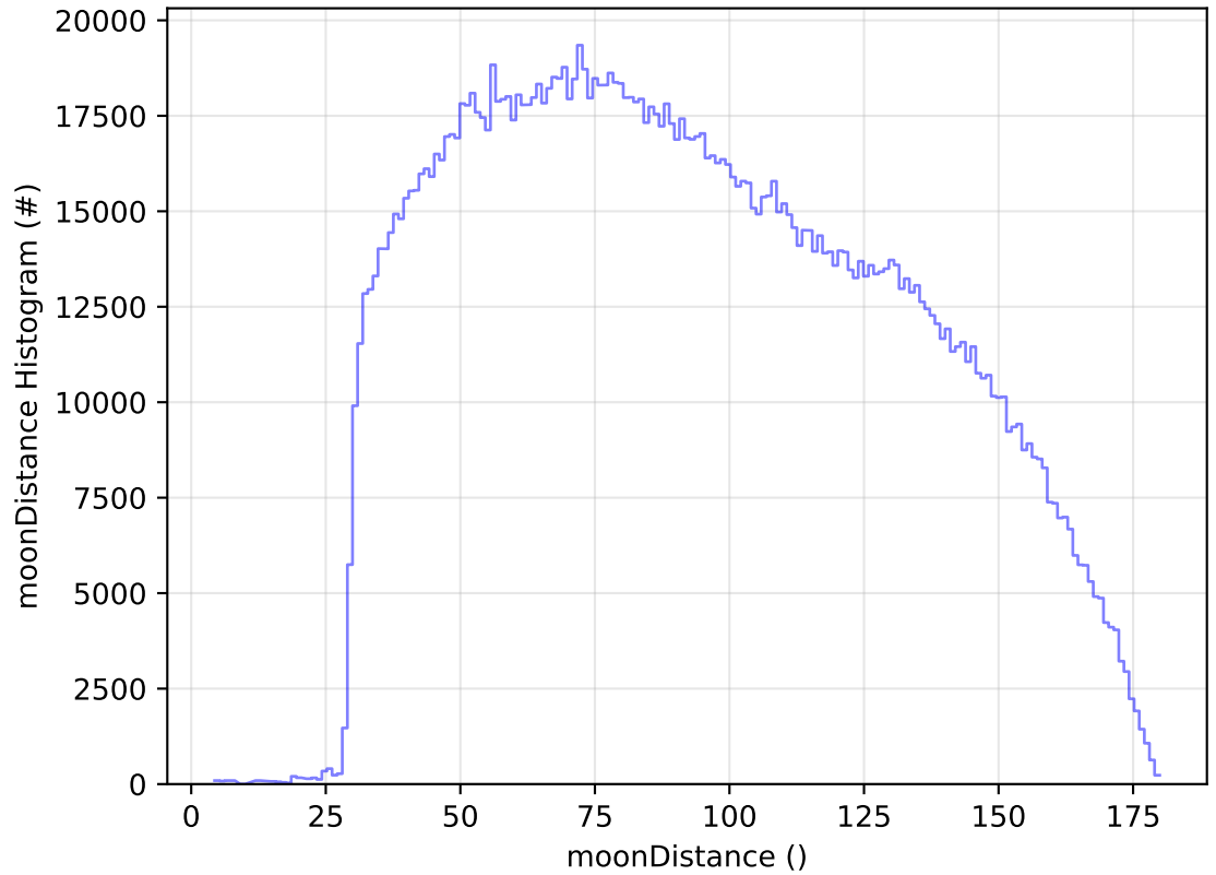
ddf_acor_sf15_lsf30_lsr50_v3.4_10yrs WFD all bands: moonDistance Histogram
