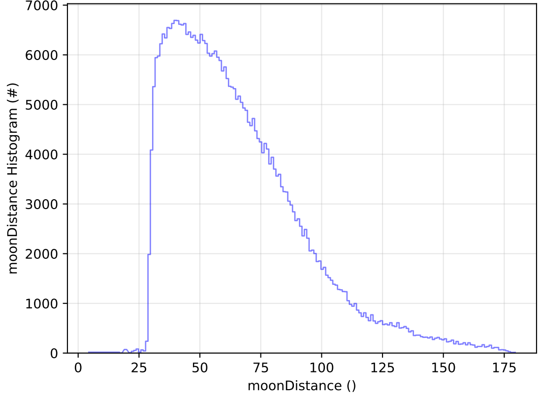
ddf_acor_sf15_lsf30_lsr50_v3.4_10yrs All sky y band: moonDistance Histogram
