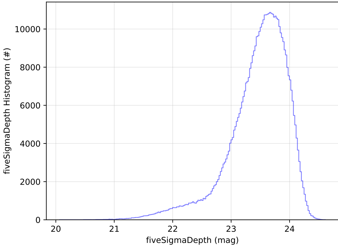
ddf_acor_sf15_lsf30_lsr50_v3.4_10yrs All sky i band: fiveSigmaDepth Histogram
