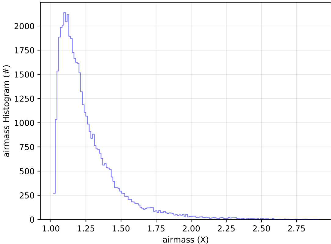
ddf_acor_sf15_lsf30_lsr50_v3.4_10yrs Yr 1 y band: airmass Histogram
