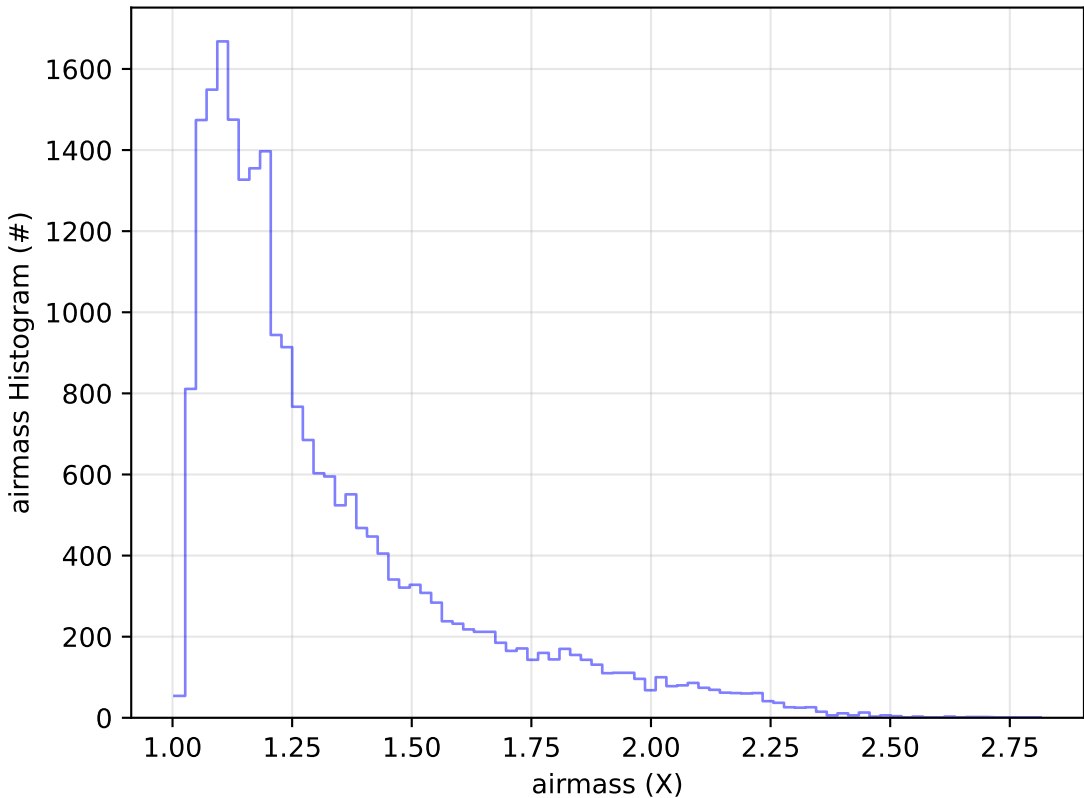
ddf_acor_sf15_lsf30_lsr50_v3.4_10yrs Yr 1 g band: airmass Histogram
