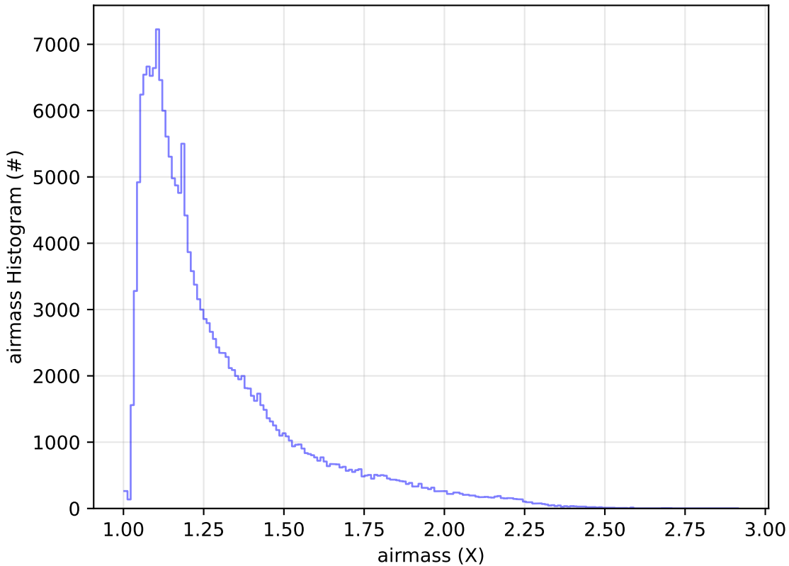
ddf_acor_sf15_lsf30_lsr50_v3.4_10yrs WFD g band: airmass Histogram
