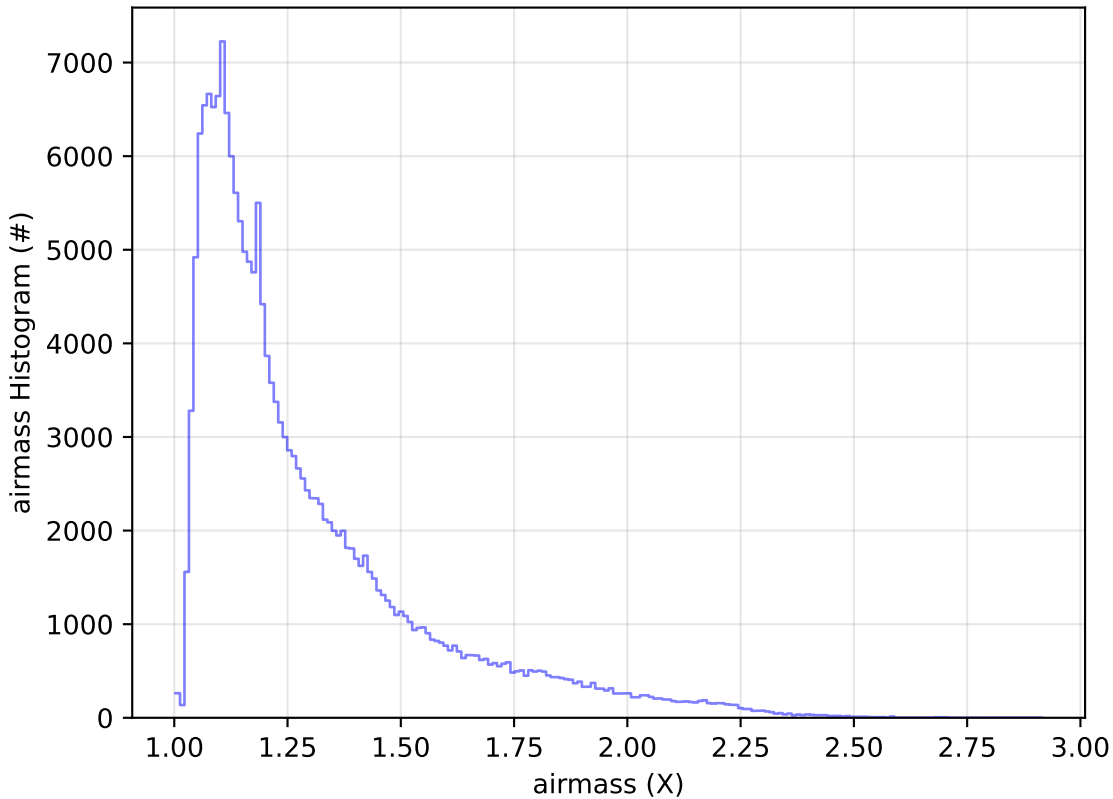
ddf_acor_sf15_lsf30_lsr50_v3.4_10yrs All sky g band: airmass Histogram
