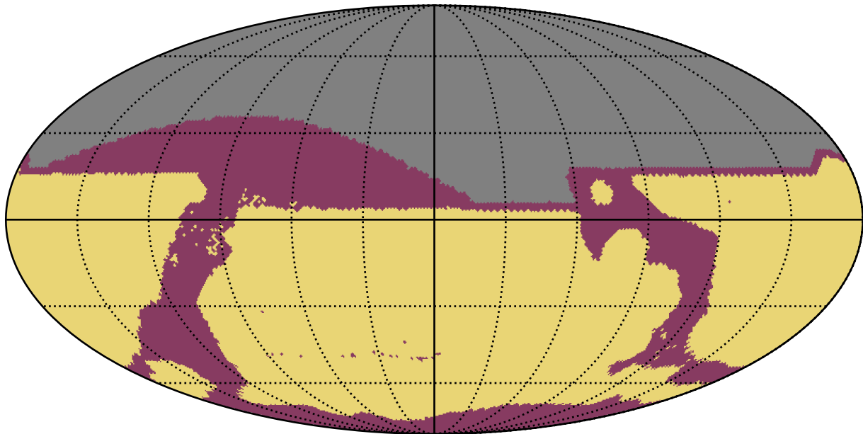
ddf_acor_sf15_lsf30_lsr50_v3.4_10yrs All sky: RapidRevisits
