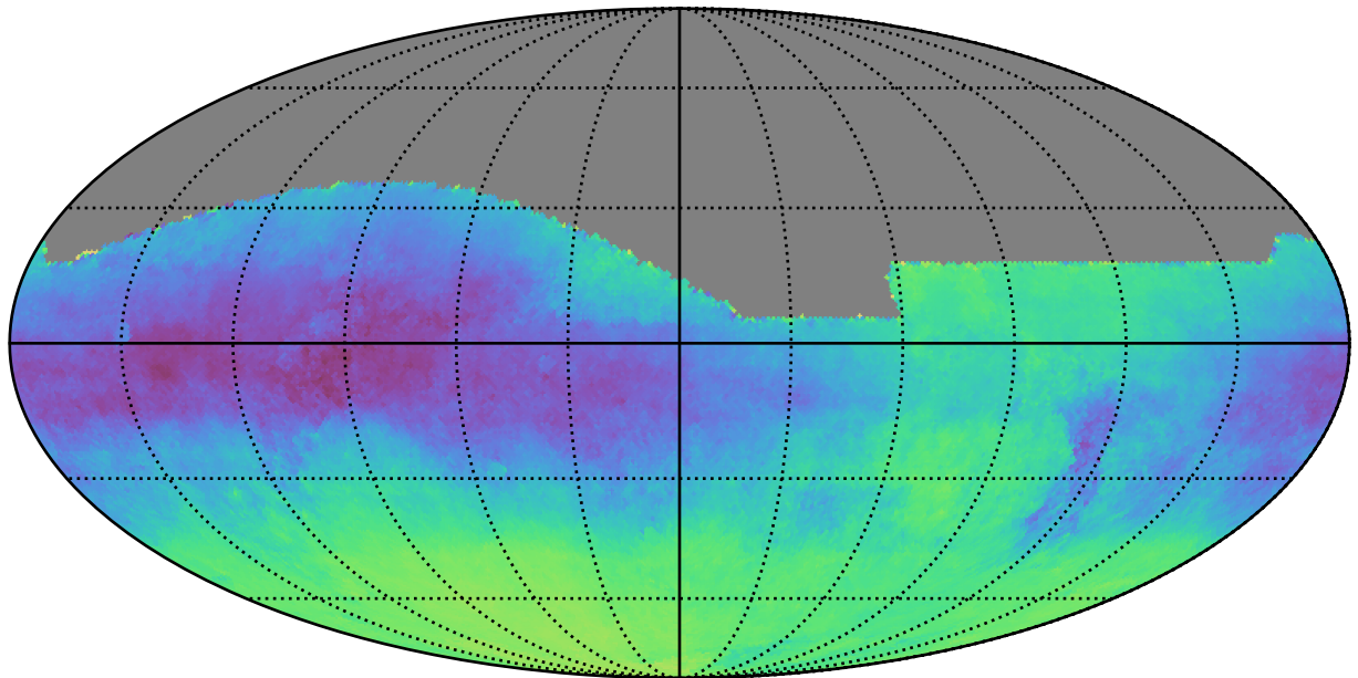
ddf_acor_sf15_lsf30_lsr50_v3.4_10yrs All sky: Parallax-DCR degeneracy @ 24.0
