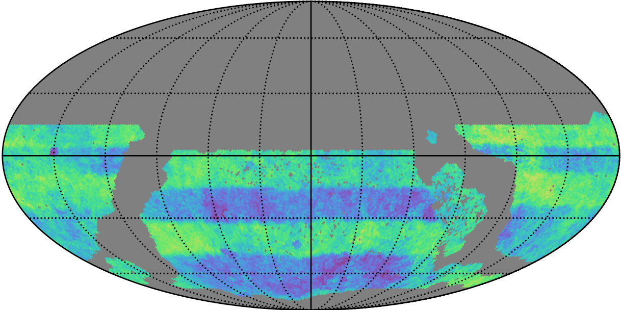
ddf_acor_sf15_lsf30_lsr50_v3.4_10yrs WFD: Normalized Proper Motion Uncert @ 24.0
