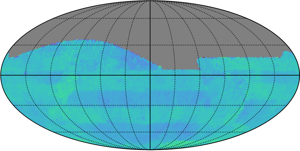
ddf_acor_sf15_lsf30_lsr50_v3.4_10yrs All sky: Normalized Proper Motion Uncert @ 24.0
