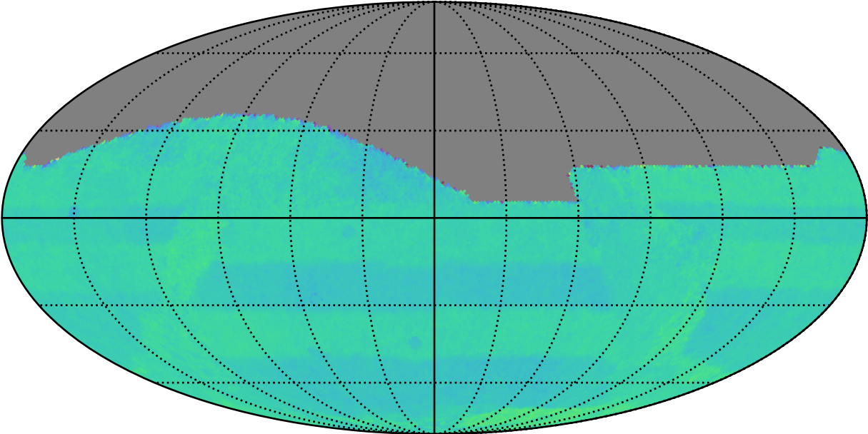
ddf_acor_sf15_lsf30_lsr50_v3.4_10yrs All sky: Normalized Proper Motion Uncert @ 20.5
