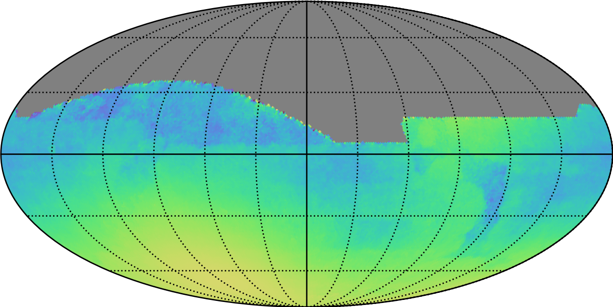
ddf_acor_sf15_lsf30_lsr50_v3.4_10yrs All sky: Normalized Parallax Uncert @ 22.4
