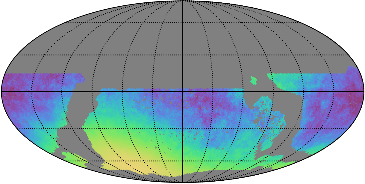
ddf_acor_sf15_lsf30_lsr50_v3.4_10yrs WFD y band only: Normalized Parallax Uncert @ 21.3
