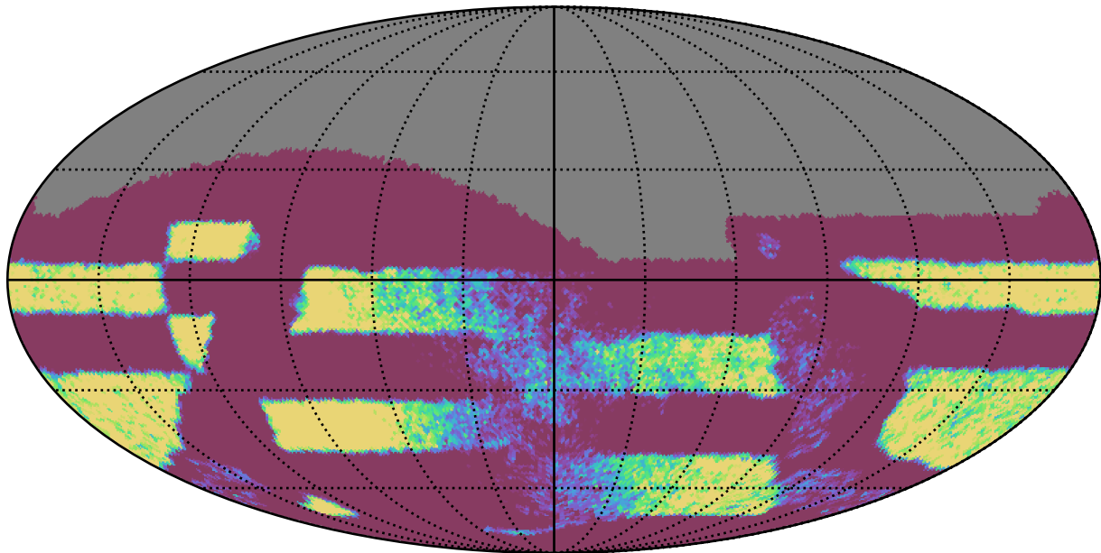
ddf_acor_sf15_lsf30_lsr50_v3.4_10yrs Yr 3-4 all bands: NVisits
