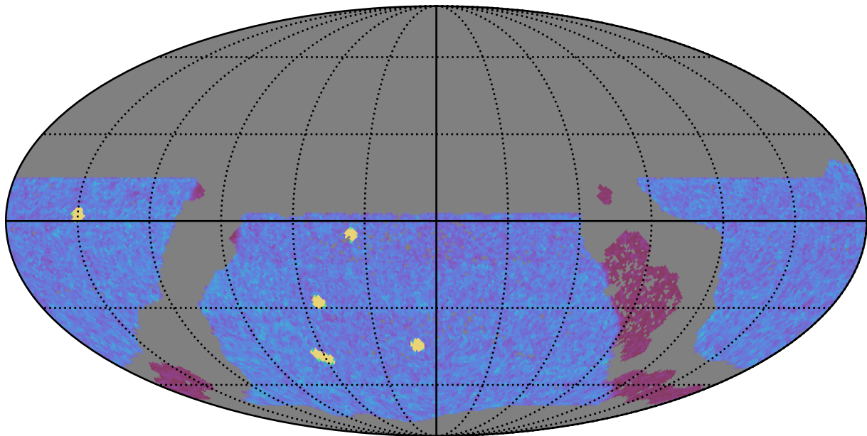
ddf_acor_sf15_lsf30_lsr50_v3.4_10yrs WFD y band: NVisits
