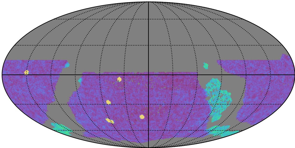
ddf_acor_sf15_lsf30_lsr50_v3.4_10yrs WFD g band: NVisits
