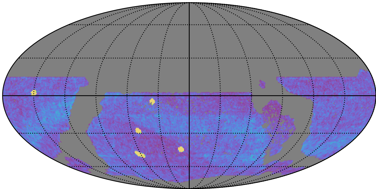
ddf_acor_sf15_lsf30_lsr50_v3.4_10yrs WFD all bands: NVisits
