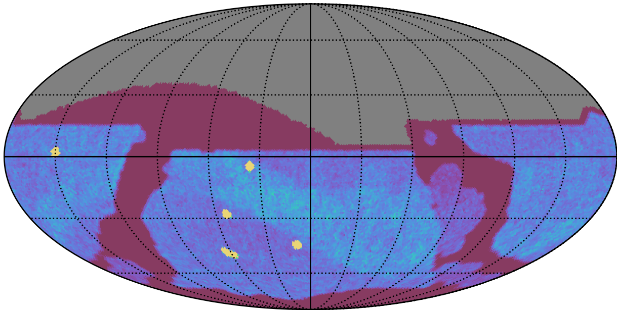
ddf_acor_sf15_lsf30_lsr50_v3.4_10yrs All sky z band: NVisits
