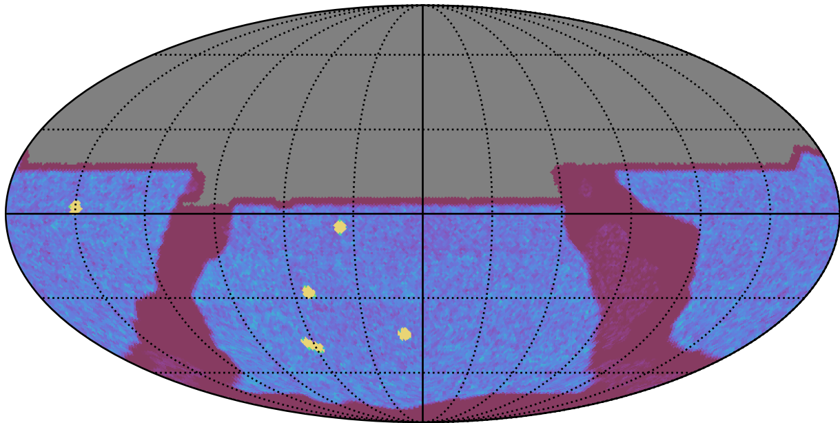
ddf_acor_sf15_lsf30_lsr50_v3.4_10yrs All sky y band: NVisits
