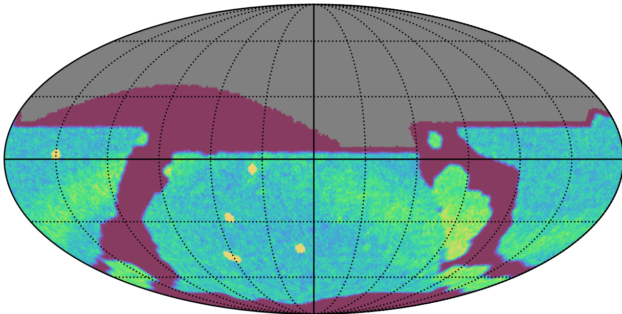
ddf_acor_sf15_lsf30_lsr50_v3.4_10yrs All sky r band: NVisits
