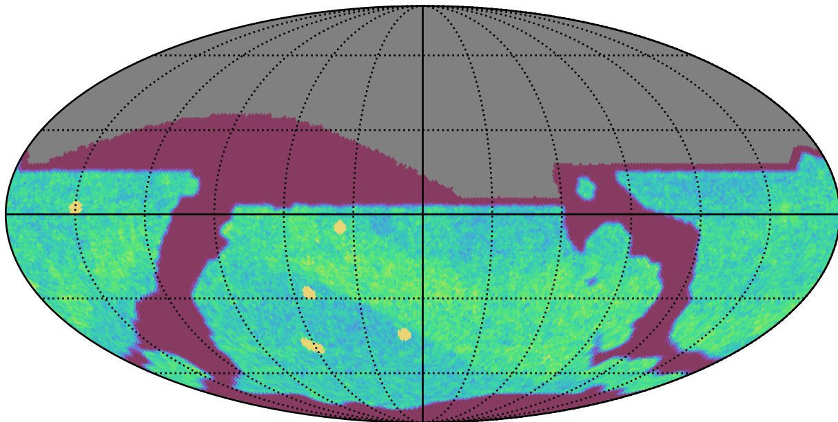
ddf_acor_sf15_lsf30_lsr50_v3.4_10yrs All sky i band: NVisits
