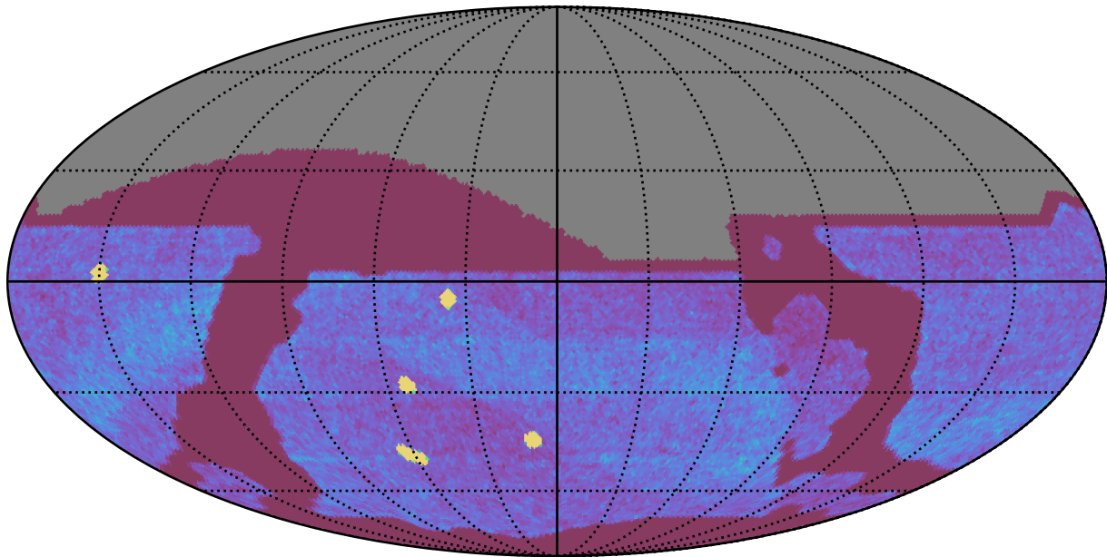
ddf_acor_sf15_lsf30_lsr50_v3.4_10yrs All sky all bands: NVisits
