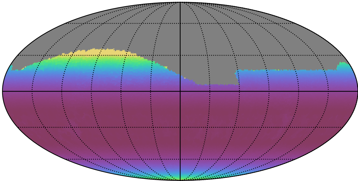
ddf_acor_sf15_lsf30_lsr50_v3.4_10yrs Yr 1 all bands: Min airmass
