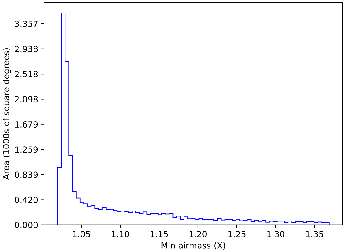
ddf_acor_sf15_lsf30_lsr50_v3.4_10yrs WFD z band: Min airmass
